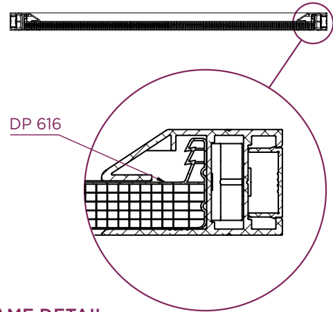
FRAME DETAIL
